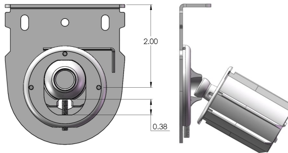
Adjustable Height Idler Bracket
