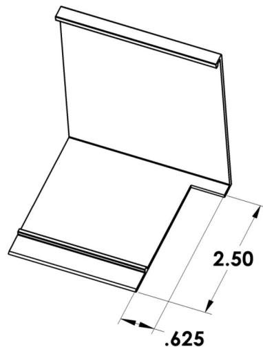
4" FASCIA PUNCH DIMENSIONS
