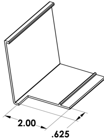
3" FASCIA PUNCH DIMENSIONS
